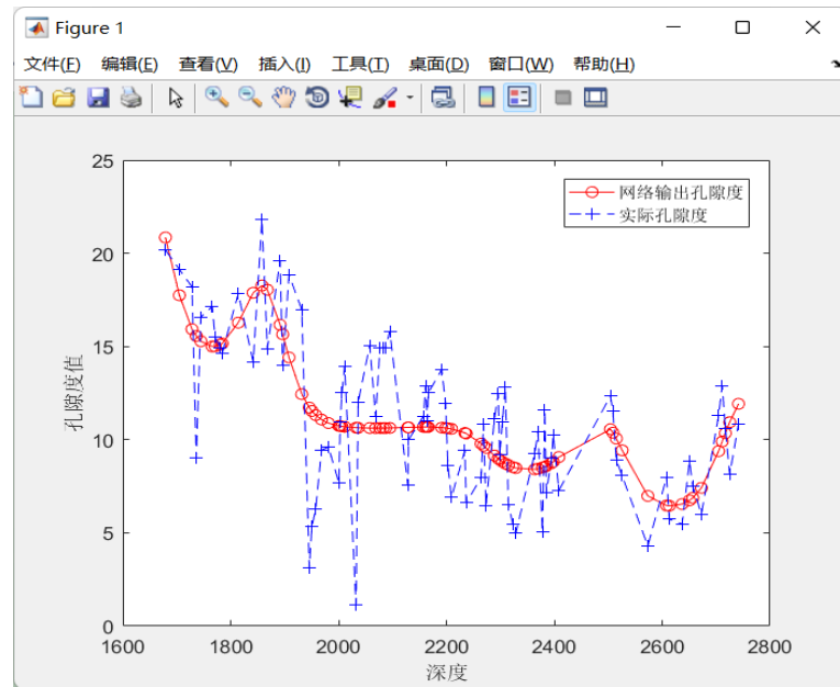
Figure 5: Comparison of predicted and actual porosity.
